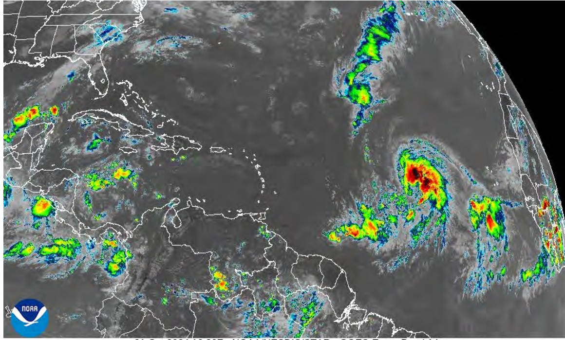
01 Oct 2024 16:30Z - NOAA/NESDIS/STAR - GOES-East - Band 14
